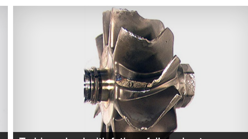
Turbine wheel with fatigue failure due to cyclic overspeed
